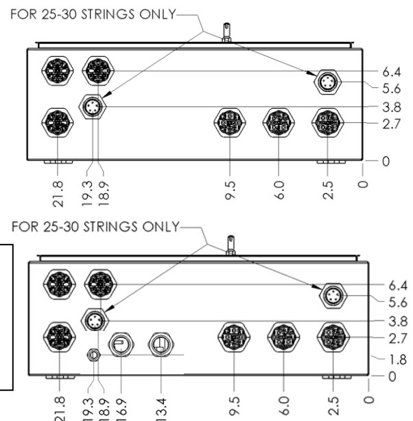
Figure 19 – Cord Grip Locations for Up to 30 Circuits
