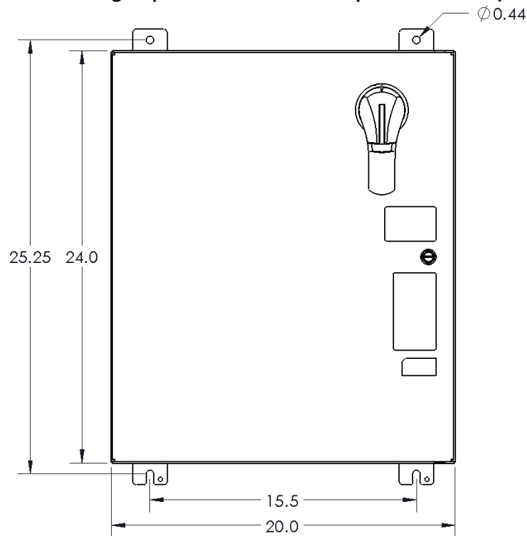
Figure 4—DISCOM 4M 13-20 Dimensions
