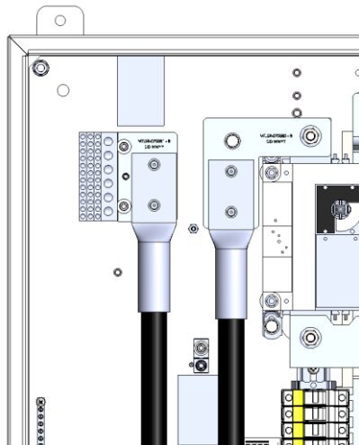
Figure 13 – Crimp Lug Option Locations (21-30 Shown)
