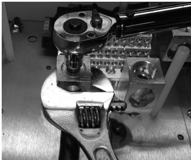
Picture 1 – Output Lug with Backup Wrench
