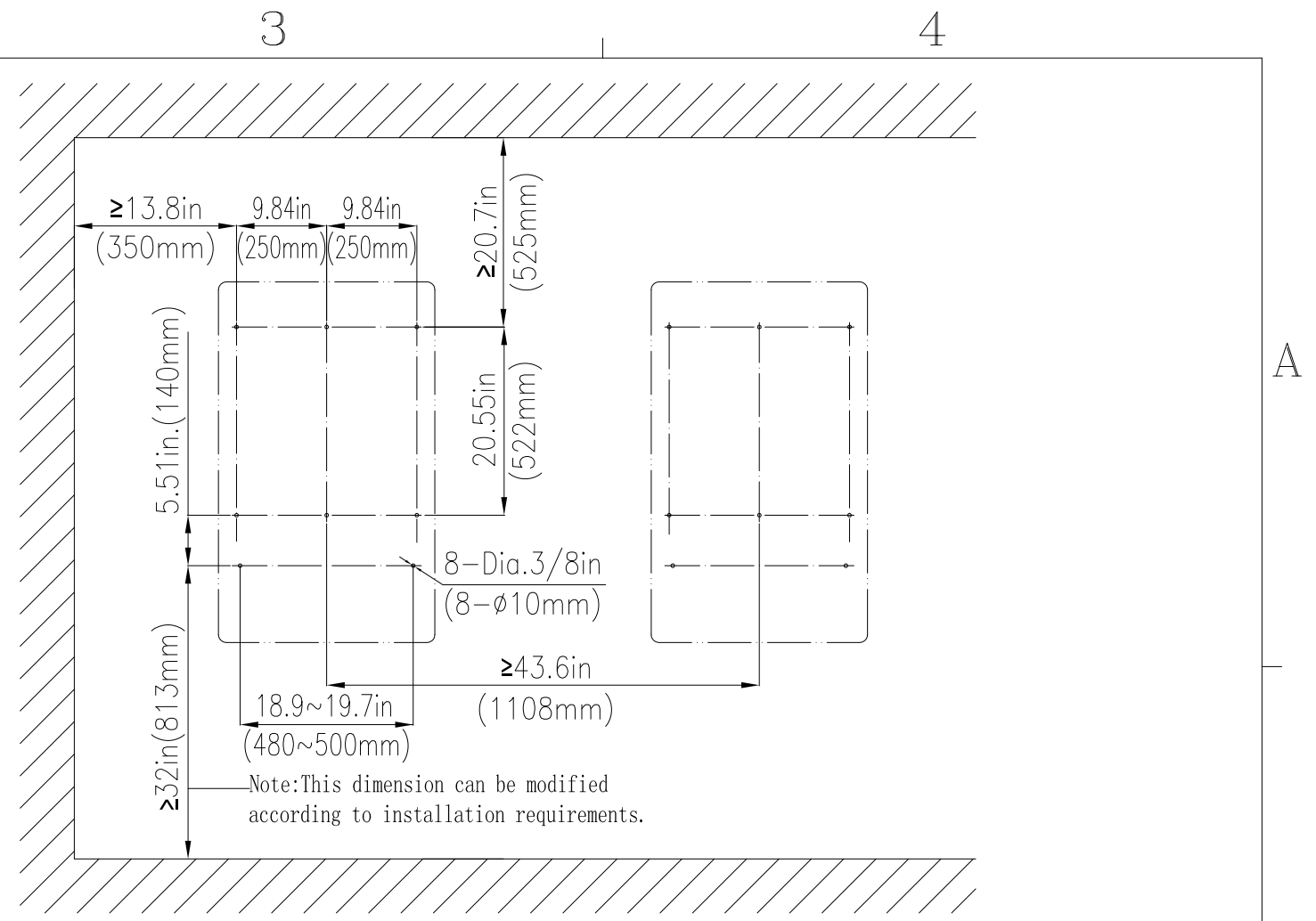
(The position of mounting holes on wall or fix bracket)
