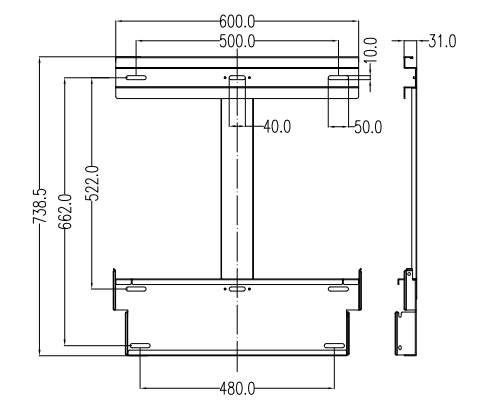
(The dimensions of mounting bracket)
