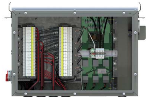
Plug & Play Wiring Box
