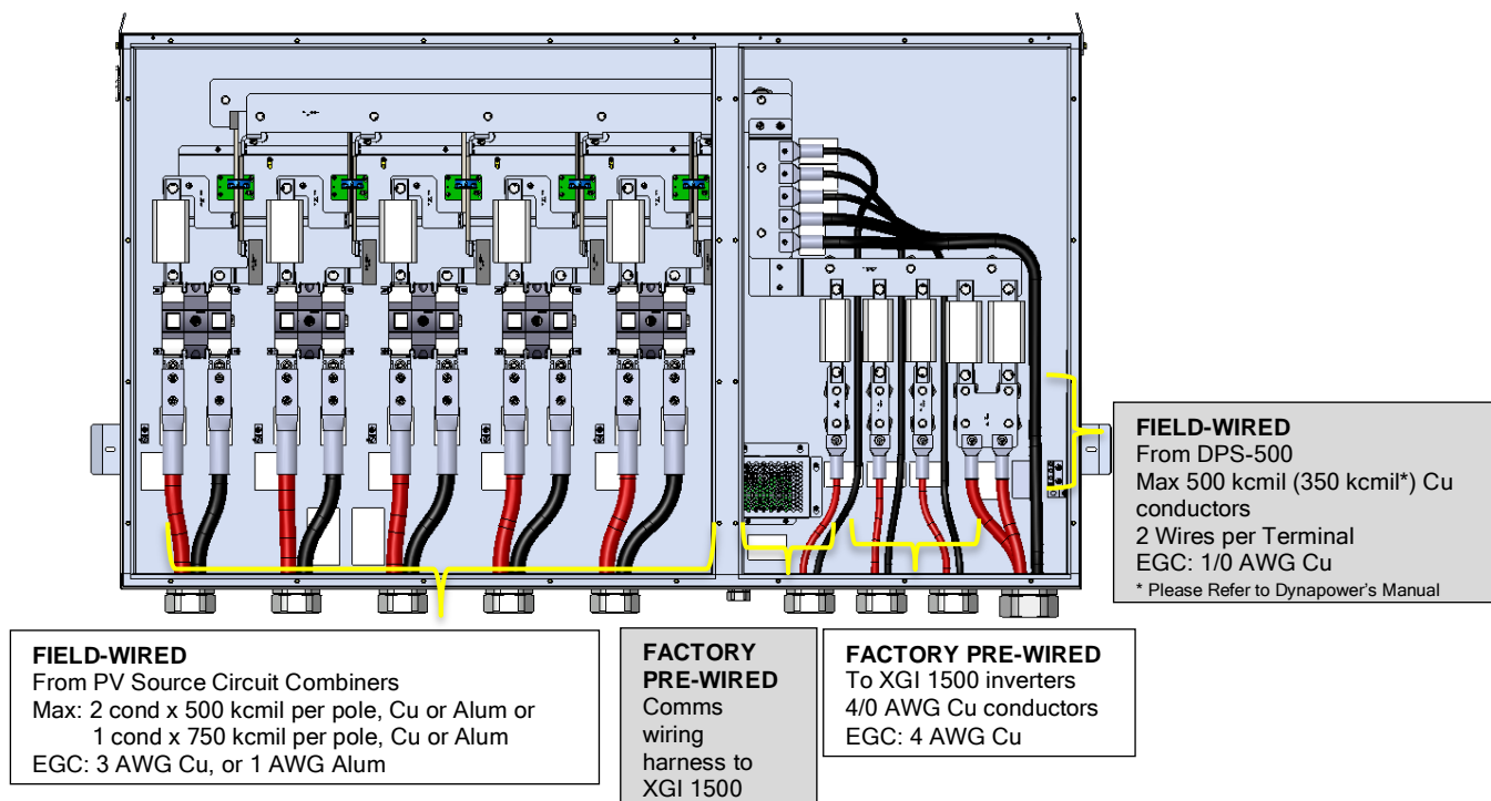
Figure 4.9 – Specs for Field Wiring to the DCR-1500 Re-Combiner
