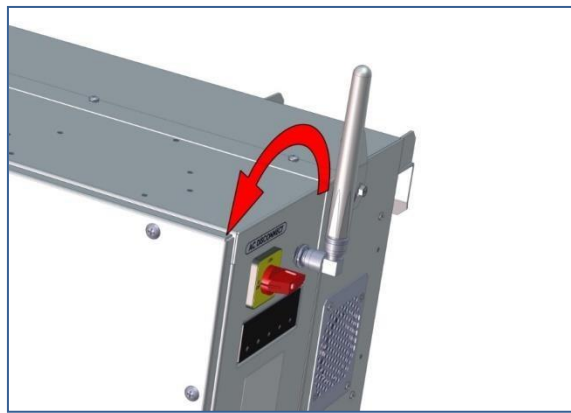
Figure 4.1 Rotate the XGI 1500 Inverter AC Disconnect to the “Off” position
