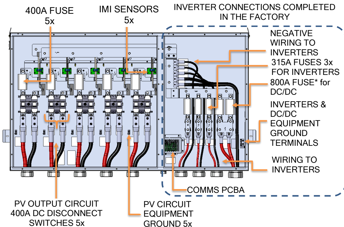
Figure 4.8 The DCR-1500 DC Re-Combiner Components
