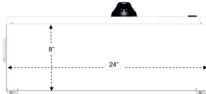
Fig 4.3 Bottom of the CR1500-400 Enclosure
