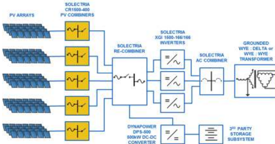
Figure 2.1 – Illustrated Usage of the CR1500-400 Combiner in the SOLECTRIA PVS-500 Energy Storage System
