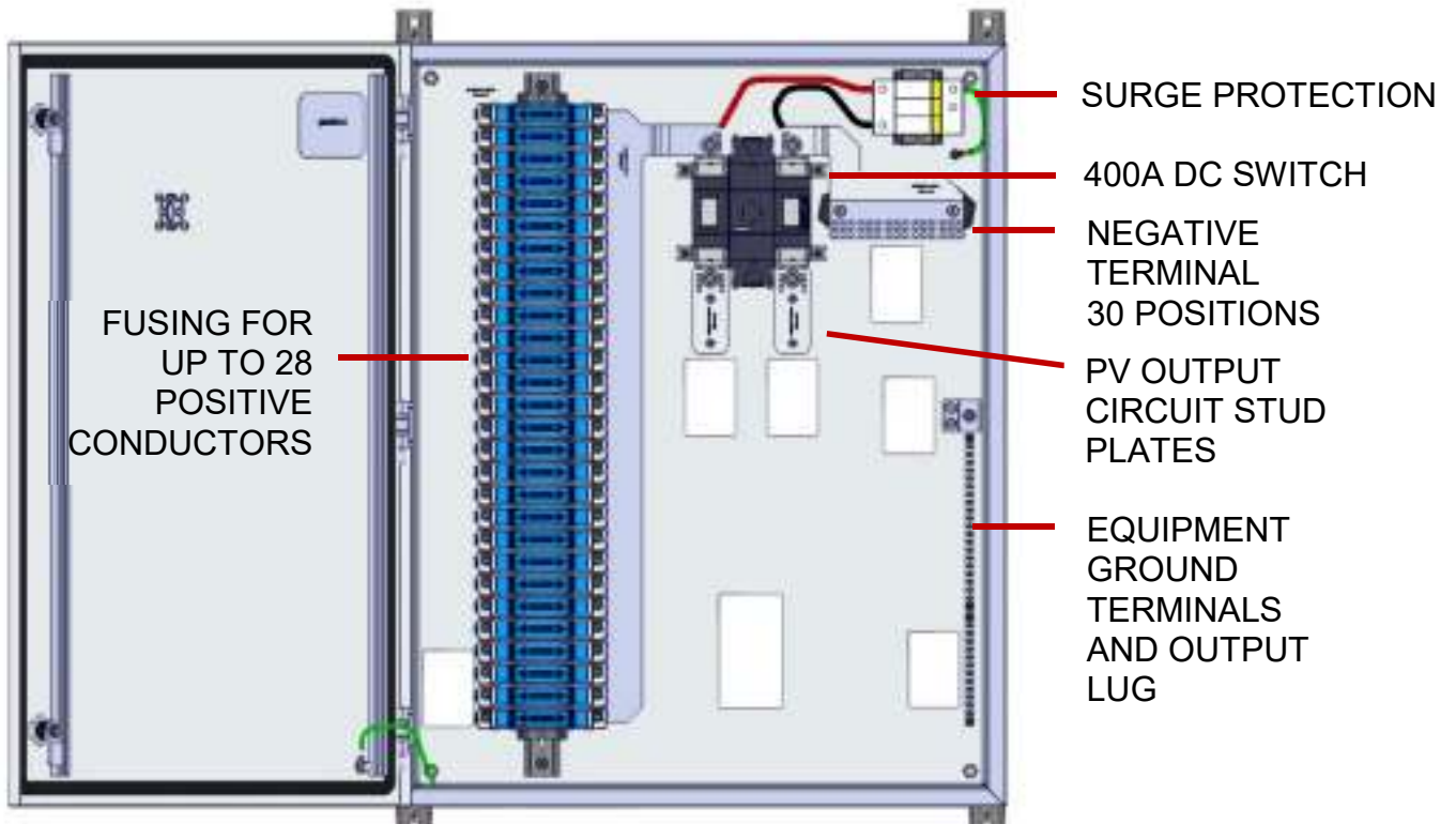
Figure 2.2 - The CR1500-400 DC Combiner
