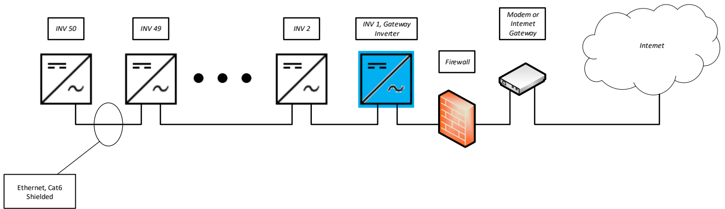
Figure 4-1 Daisy Chain
