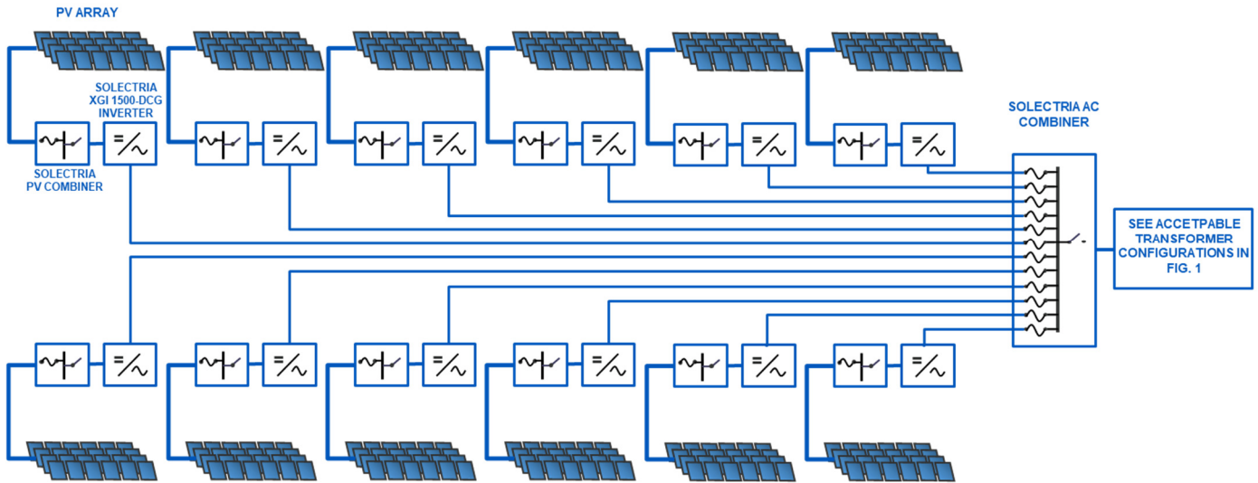
Figure 2. Maximum number of 12 XGI 1500-DCG inverters per transformer winding
