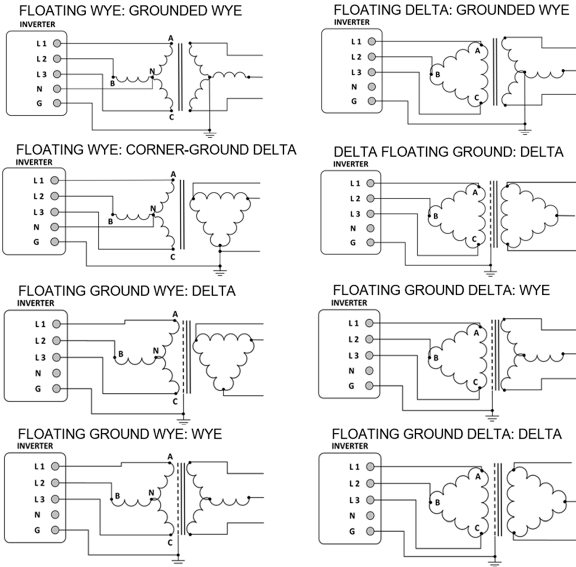
Figure 1. Permitted Transformer Configurations for XGI 1500-DCG Interconnection
